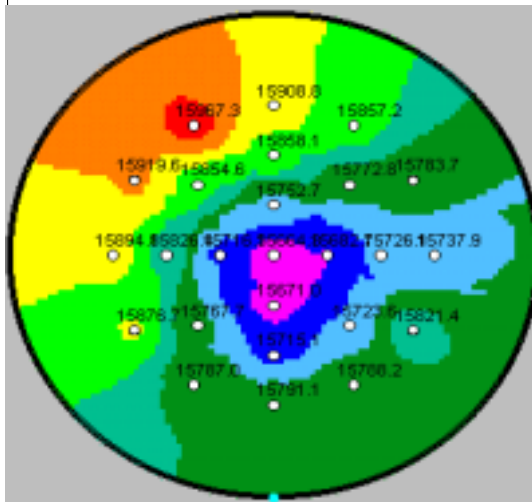
BEFORE STRIP
